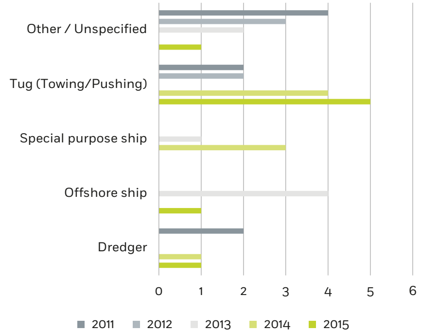
Figure 121: Distribution of fatalities per service ship type
