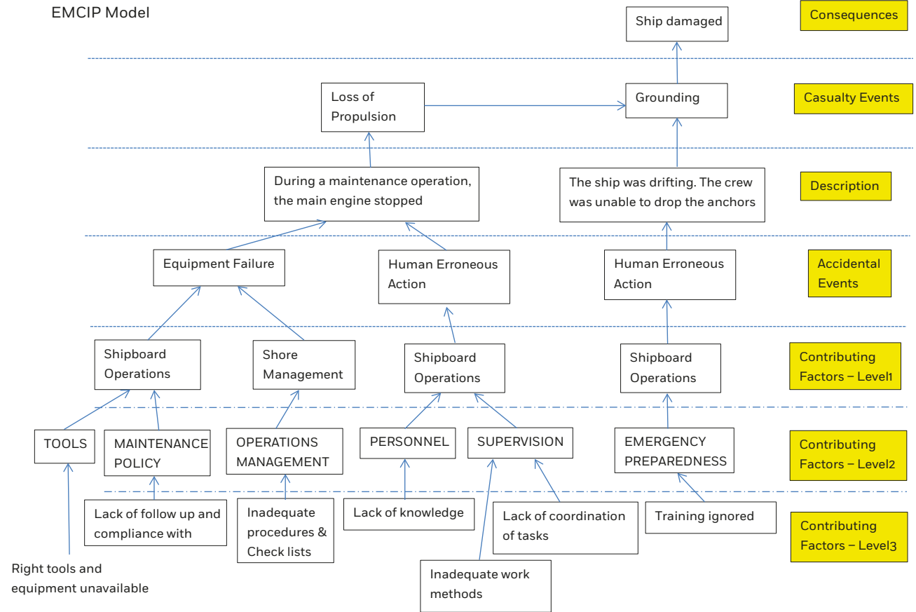
Figure 152: EMCIP Model
